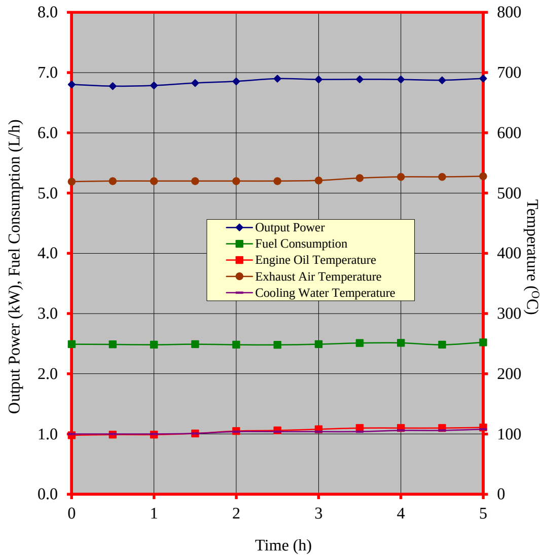
Figure 4. Performance characteristic curves during the continuous running test of the PLATINUM PT95 KNM950 diesel engine
