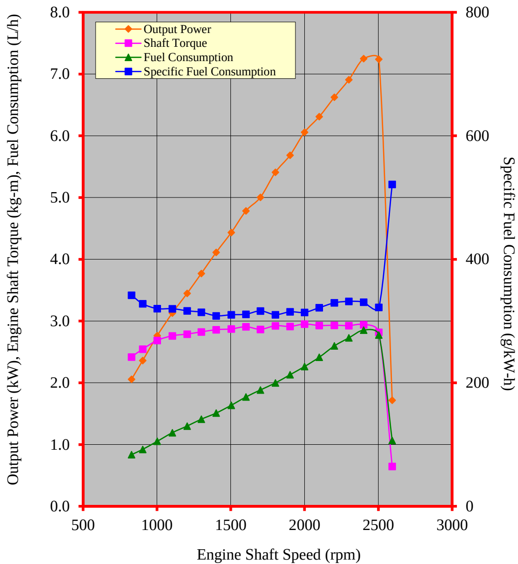
Figure 3. Performance characteristic curves of the PLATINUM PT95 KNM950 diesel engine
